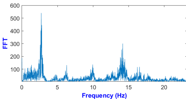
Fig. 9 Fast Fourier Transform of the acceleration at first floor
