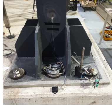
(b) Accelerometers at base joint.
