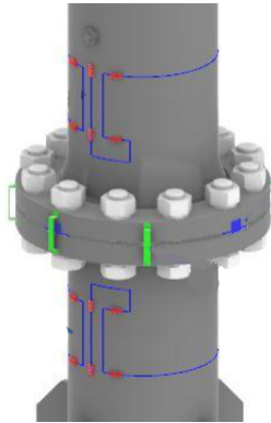
(a) FBG sensors.
